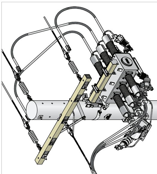
Load Break Switch
