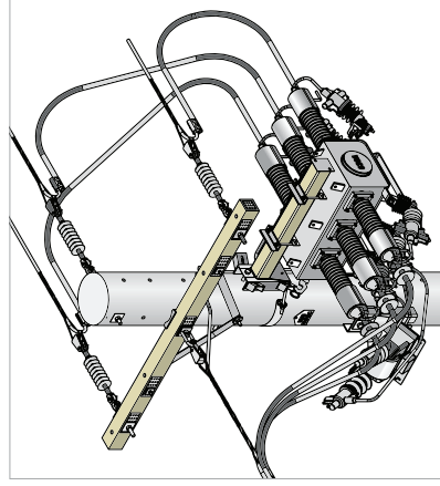
Load Break Switch
