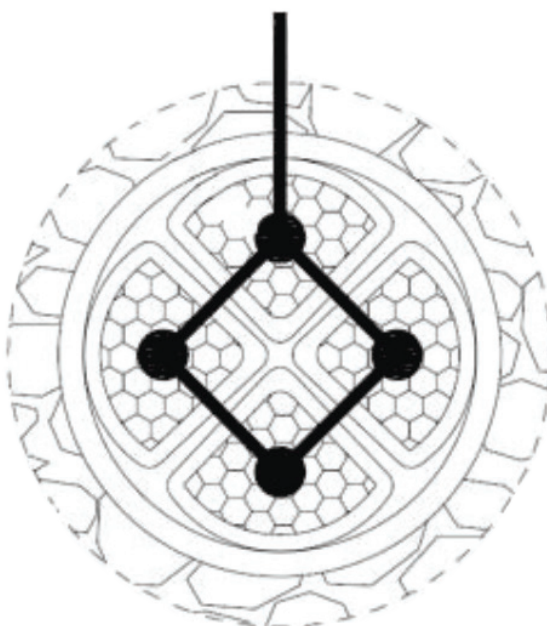
End view of cable cores bridged together
